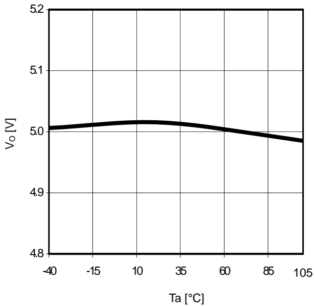
Figure 21. T_a - V_o ( I_o=0\text{mA} )
