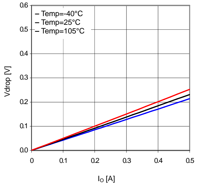
Figure 38. Minimum dropout Voltage 5 ( V_{CC}=12.0V )
