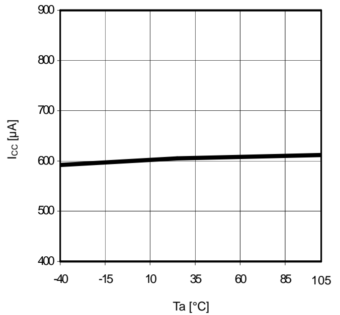
Figure 22. T_a - I_{cc}
