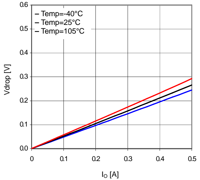
Figure 36. Minimum dropout Voltage 3 ( V_{CC}=8.0V )
