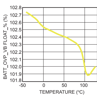
BATT_OVP_VB Float_% vs. Temperature
