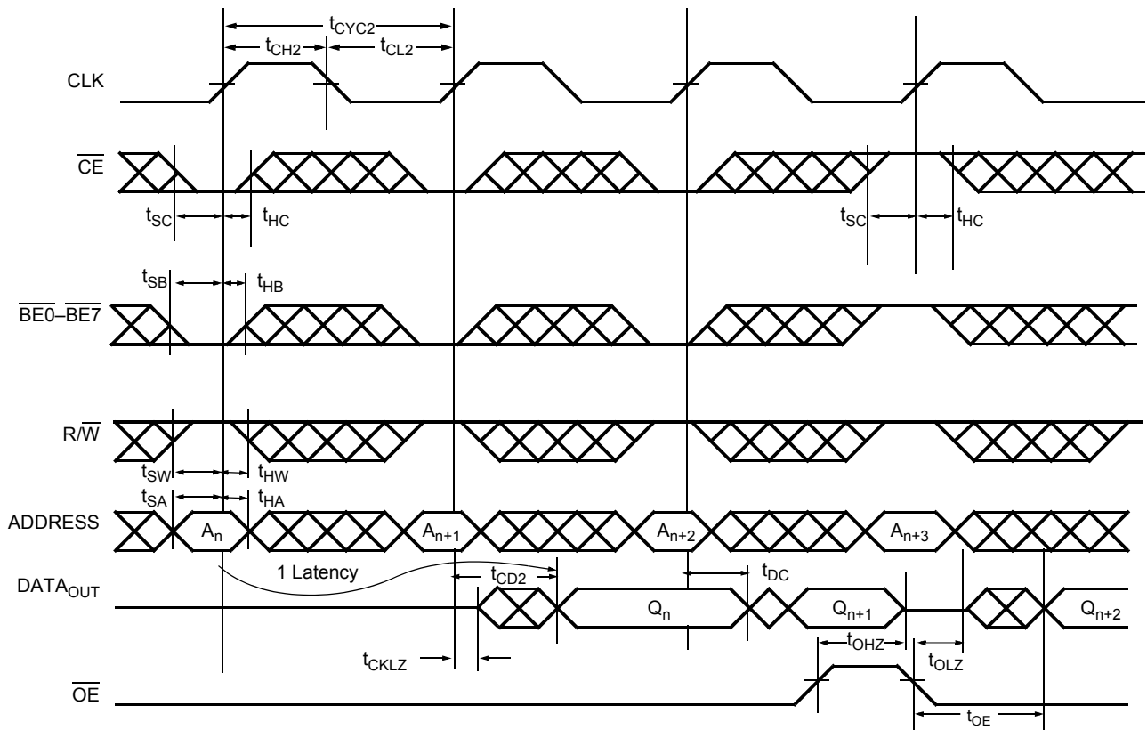
Figure 5. Read Cycle [42, 43, 44, 45, 46]
