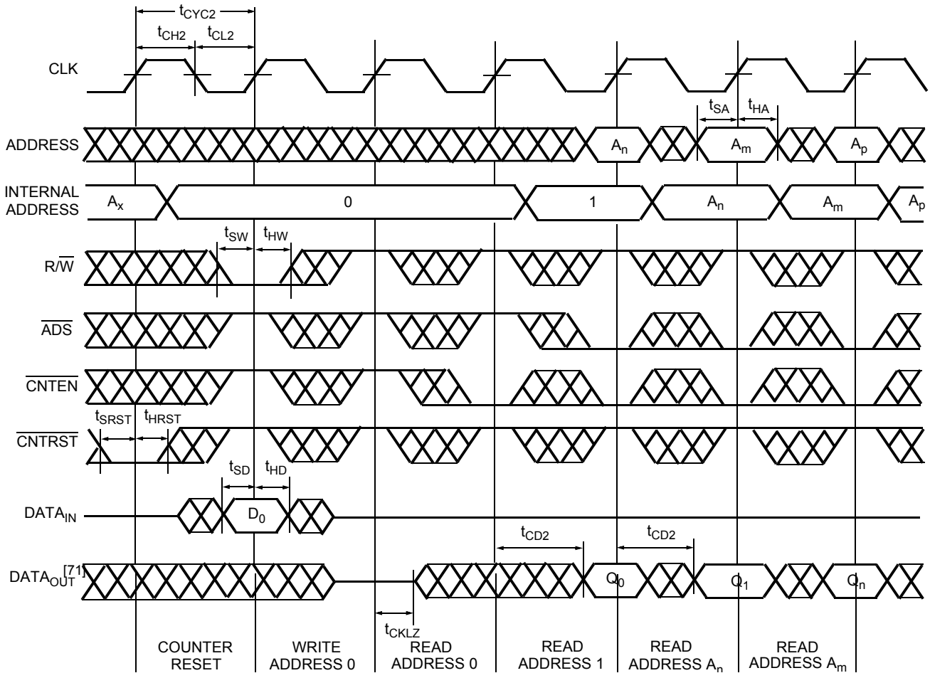
Figure 11. Counter Reset [58, 59]
