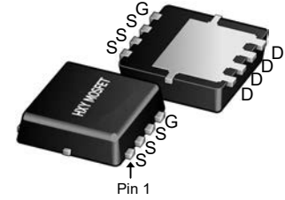
DFN3X3-8L (WDFN-8(3.3x3.3))
