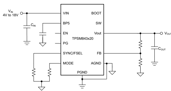
Simplified Schematic
