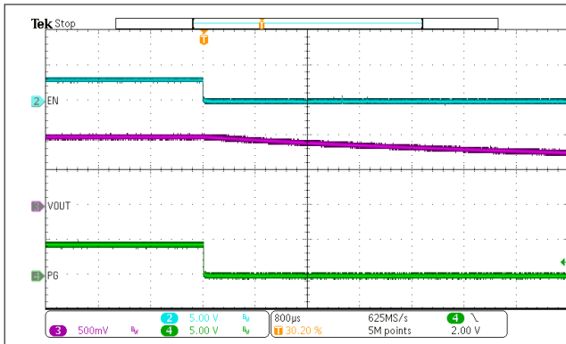
Figure 7-10. EN Shutdown No Load
