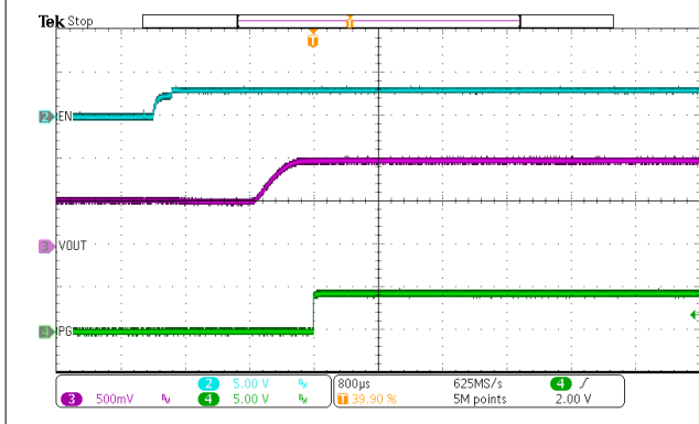
Figure 7-12. EN Start-Up – 0.5V Prebias
