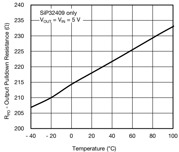
Figure 15 - Output Pulldown Resistance vs. Temperature
