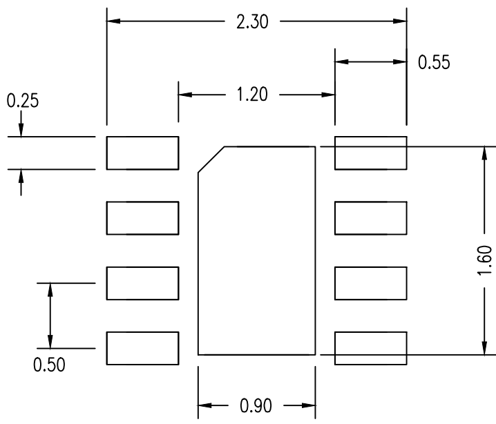
RECOMMENDED LAND PATTERN DIMENSION
