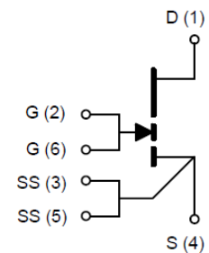
Circuit Symbol
