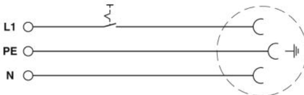
Circuit diagram
