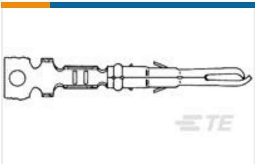
TE Part #640545-2 MR SPLIT PIN 26-18 AUPHBRZ LP
