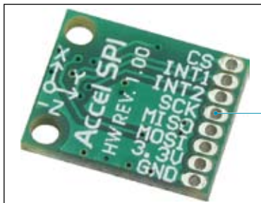
Figure 2: Accel SPI Board's back side
