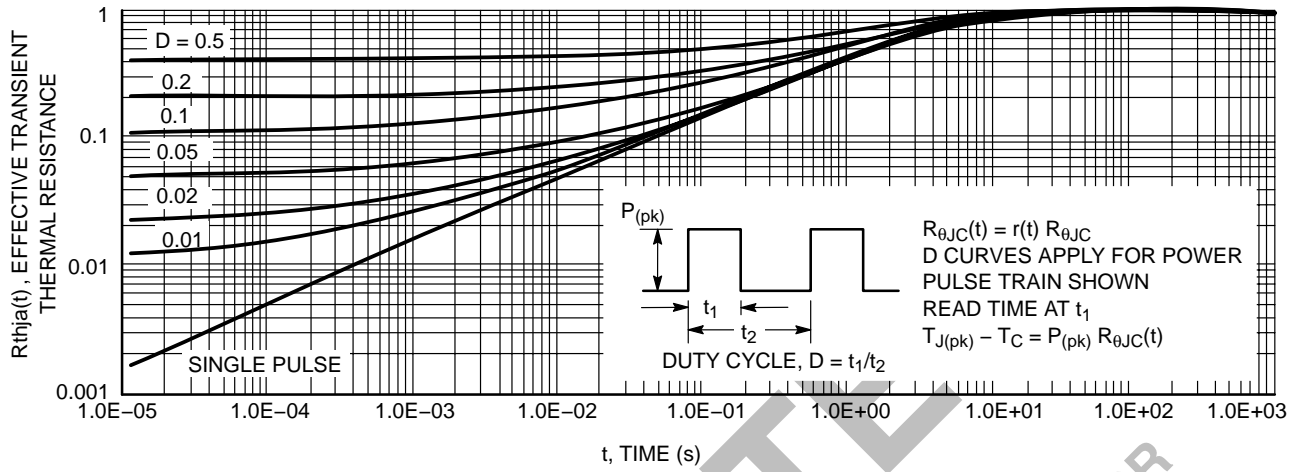
Figure 13. Thermal Response
