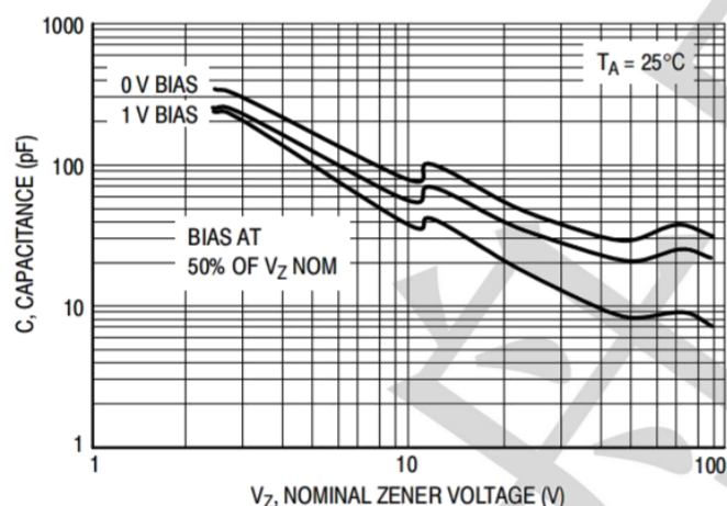
Typical Capacitance
