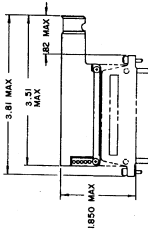
2 INCH PLUG ASSY INSTALLATION DATA REF
