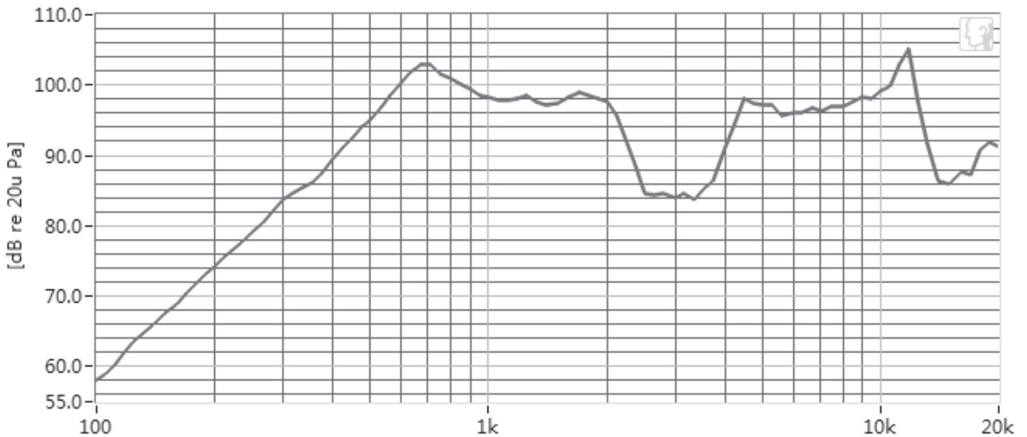
Frequency Response.Magn dB re 20.00μ PA (at 1 W / 0.1 m)
