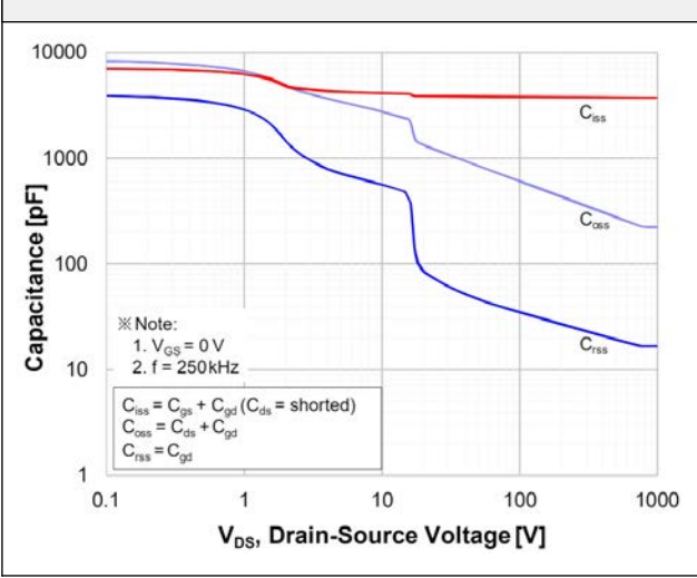
Figure 12. Capacitance Characteristics
