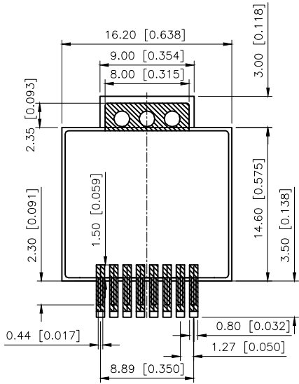
RECOMMENDED PCB LAYOUT VIEWED FROM COMPONENT SIDE
