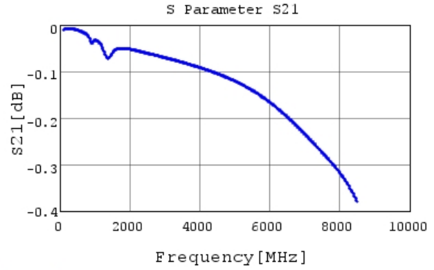
GRM1552C1H391JA01 S21 DCOV, 20degC
