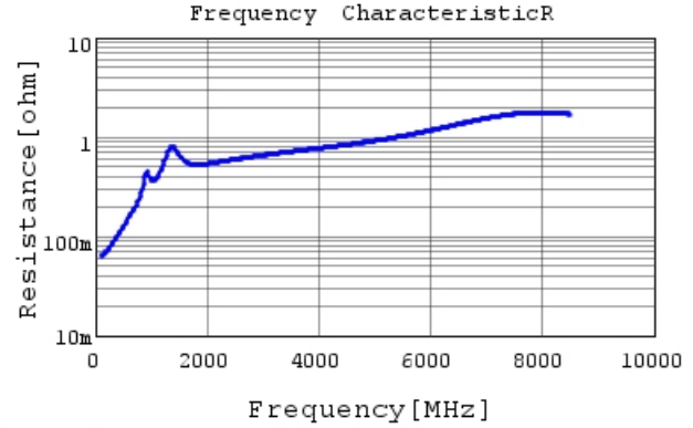
GRM1552C1H391JA01 R DCOV, 20degC
