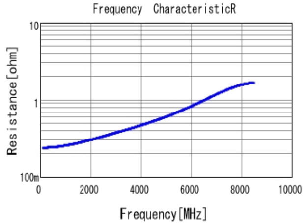
■ GRM0335C1H3R6CA01 R DC0V, 25degC
