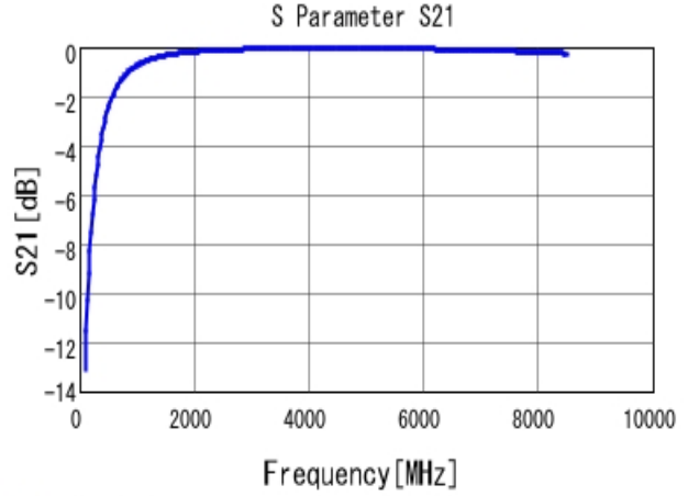
■ GRM0335C1H3R6CA01 S21 DCOV, 25degC
