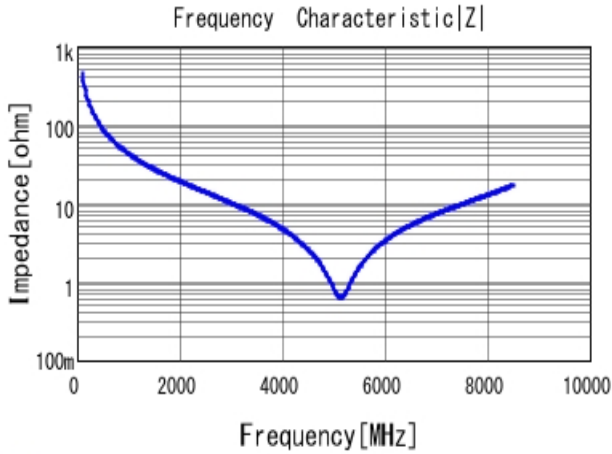
■ GRM0335C1H3R6CA01 |Z| DC0V, 25degC
