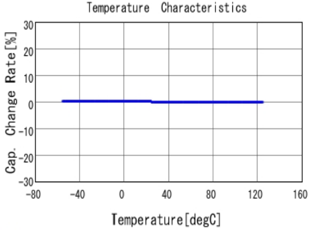
■ GRM0335C1H3R6CA01 C-Temp. capchange, DCOV, AC1Vrms
