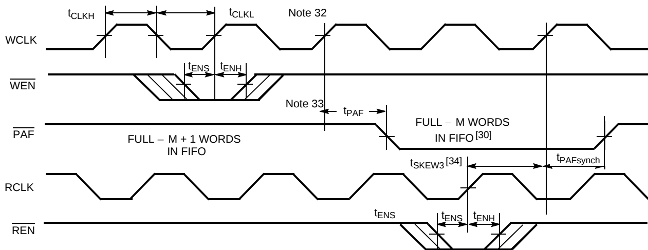
Figure 16. Programmable Almost Full Flag Timing (applies only in \overline{\text{SMODE}} ( \overline{\text{SMODE}} in LOW))
