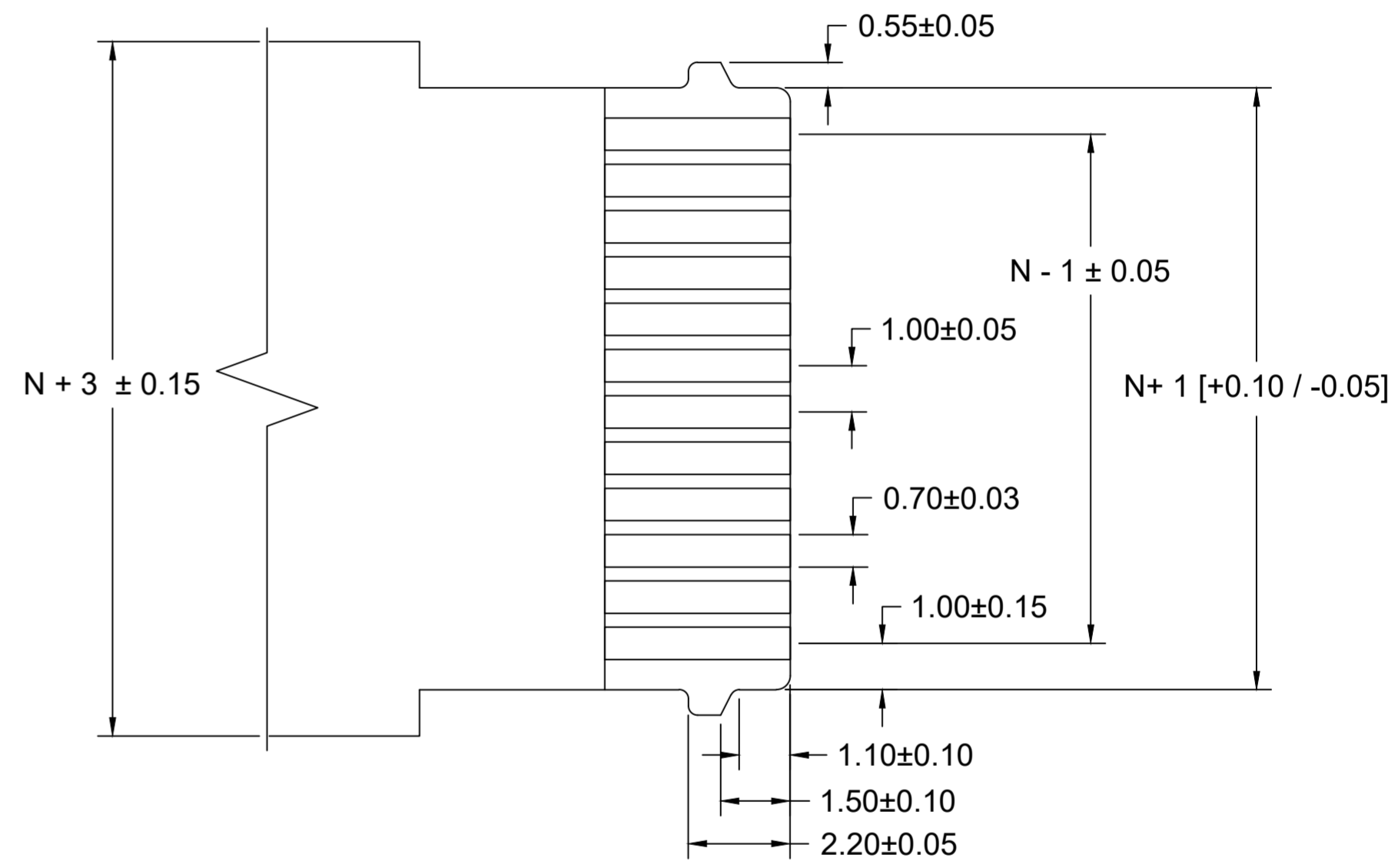
END-TAIL DIMENSIONS SCALE 10:1
