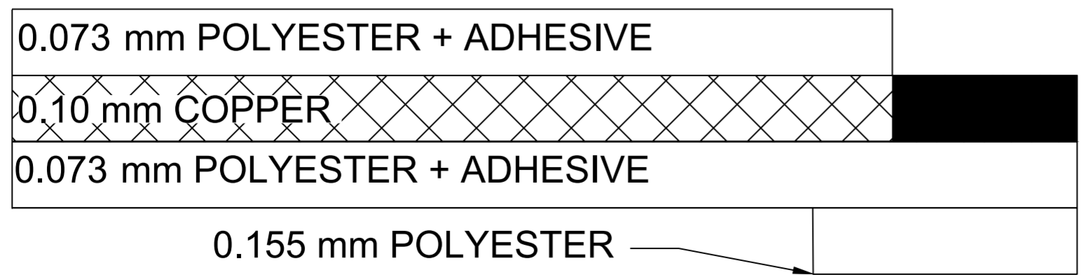
CROSS-SECTION
