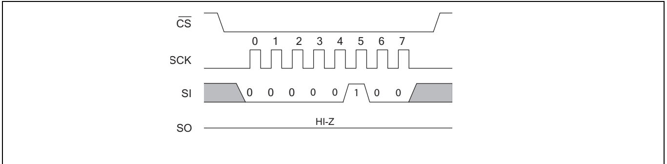
Figure 7 WRDI bus configuration
