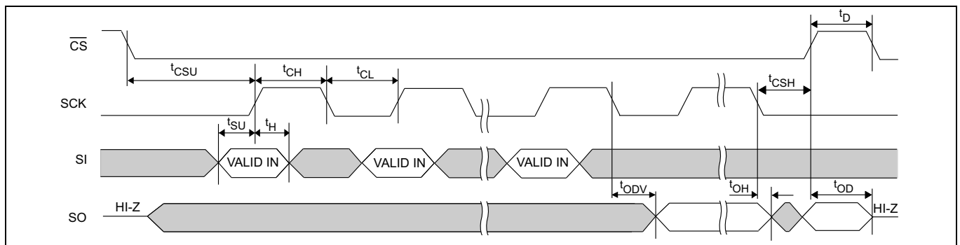
Figure 15 Synchronous data timing (Mode 0)
