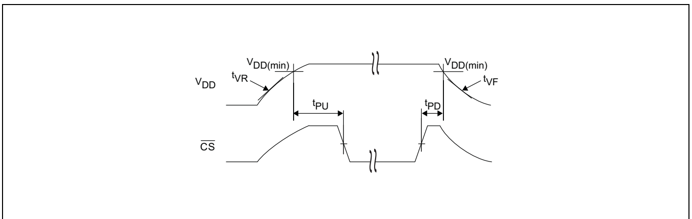
Figure 16 Power cycle timing
