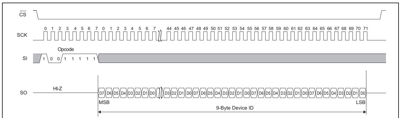
Figure 14 Read device ID
