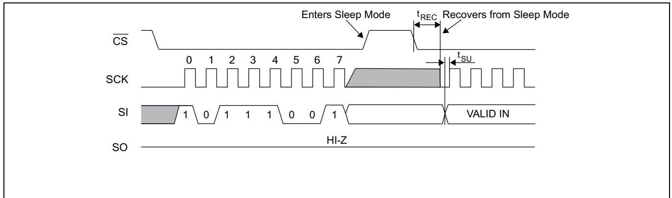
Figure 13 Sleep mode operation
