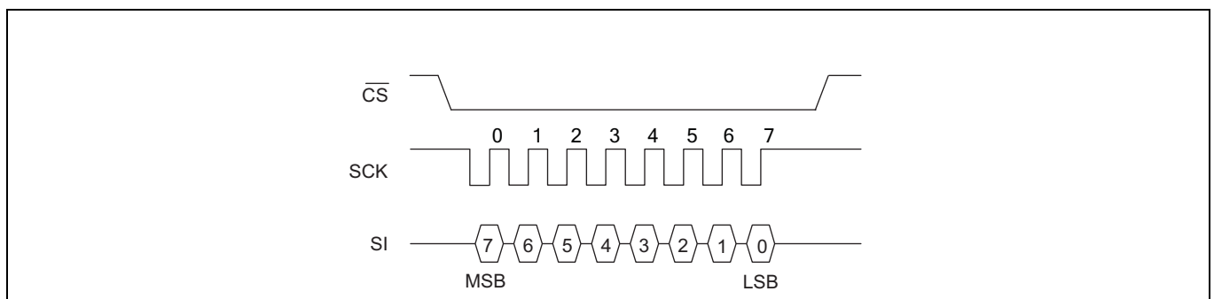
Figure 5 SPI Mode 3
