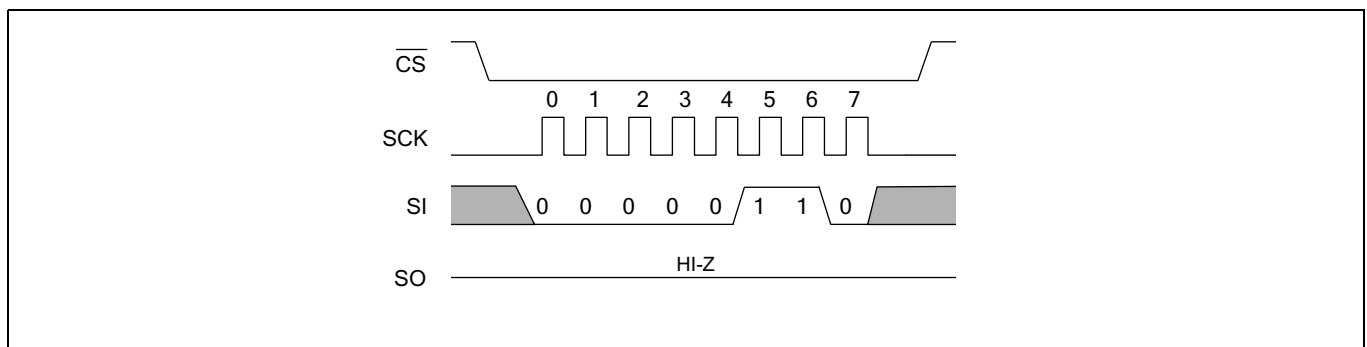
Figure 6 WREN bus configuration
