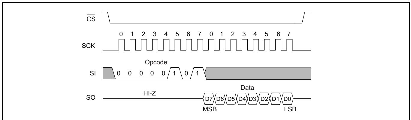
Figure 8 RDSR bus configuration
