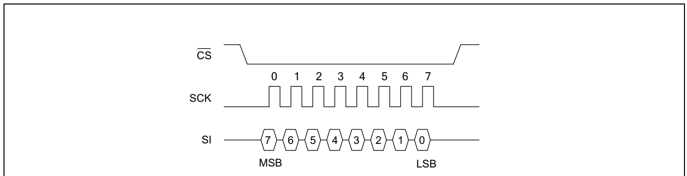
Figure 4 SPI Mode 0
