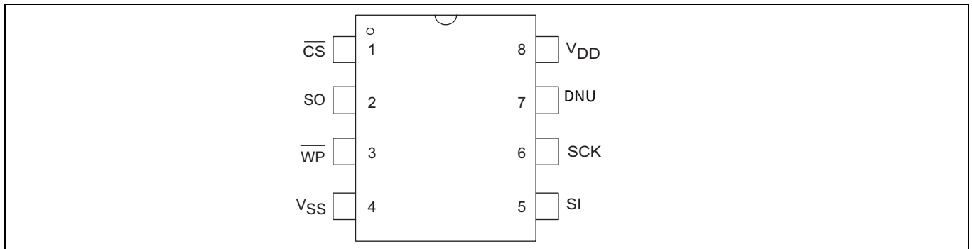
Figure 1 8-pin PDIP pinout
