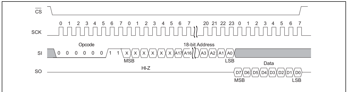
Figure 11 Memory read operation
