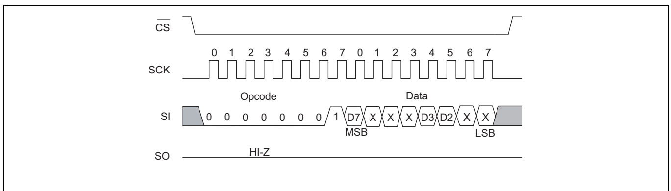
Figure 9 WRSR bus configuration (WREN not shown)
