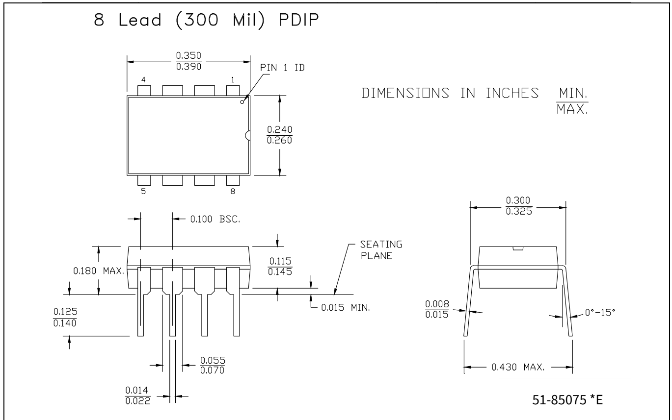
Figure 17 8-pin PDIP (300 Mils) package outline (PG-DIP-8), 51-85075
