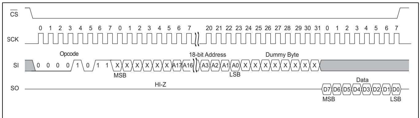
Figure 12 Fast read operation
