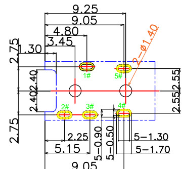
PCB LAYOUT (TOP VIEW) TOLERANCE: ±0.05
