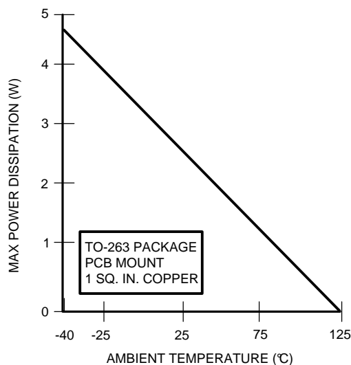
Figure 55. Derating Curve for DDPACK package. No Air Flow
