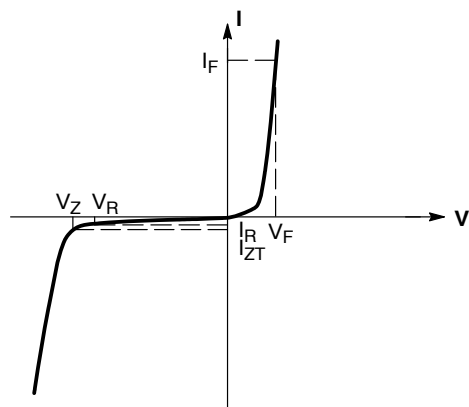
Figure 1. Uni-directional Zener
