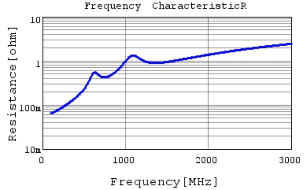
GRM31A7U2J681JW31 R DC0V, 25degC
