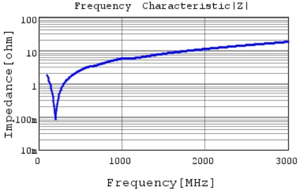
GRM31A7U2J681JW31 |Z| DC0V, 25degC
