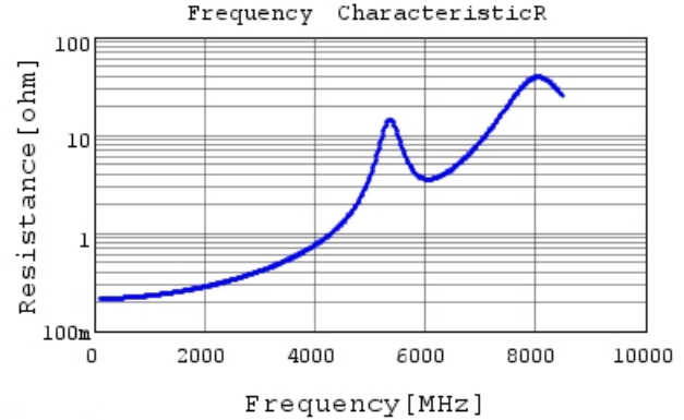
GCM1885C2A8R0BA16 R DCOV,25degC
