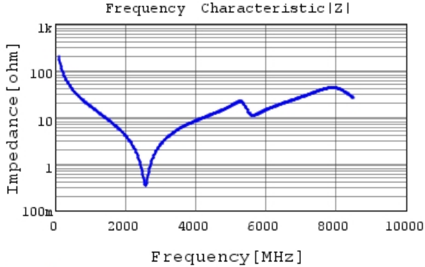
GCM1885C2A8R0BA16 |Z| DCOV,25degC
