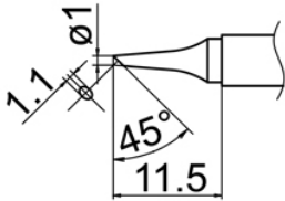
T12-BCF1 Shape-1BC Tinned cut surface only
