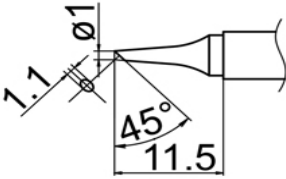
T12-BC1 Shape-1BC
