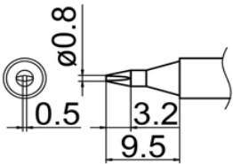
T12-D08 Shape-0.8D
