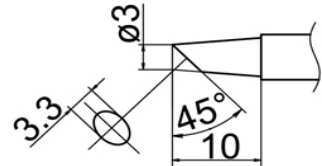
T12-BCF3 Shape-3BC Tinned cut surface only
