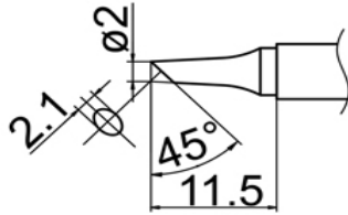
T12-BC2 Shape-2BC
