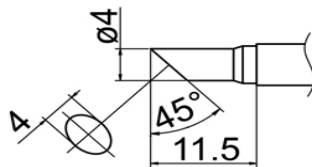
T12-CF4 Shape-4C Tinned cut surface only
