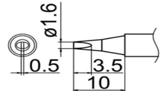
T12-D16 Shape-1.6D
