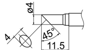
T12-C4 Shape-4C
