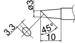
T12-BC3 Shape-3BC
