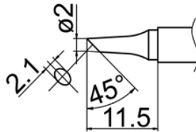
T12-BCF2 Shape-2BC Tinned cut surface only
