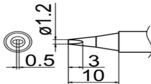
T12-D12 Shape-1.2D
