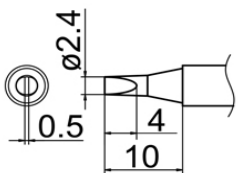
T12-D24 Shape-2.4D
