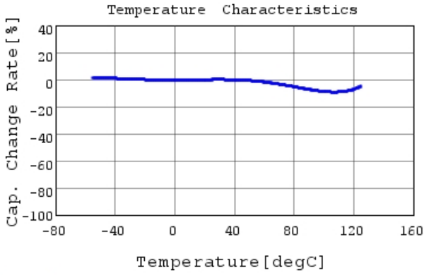
GRM55DR72A105KA01 C-Temp. capchange, DC0.0V,
