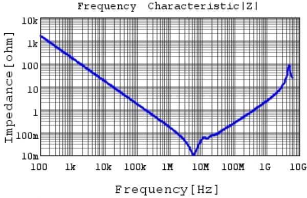
GRM55DR72A105KA01 |Z| DCOV, 25degC
