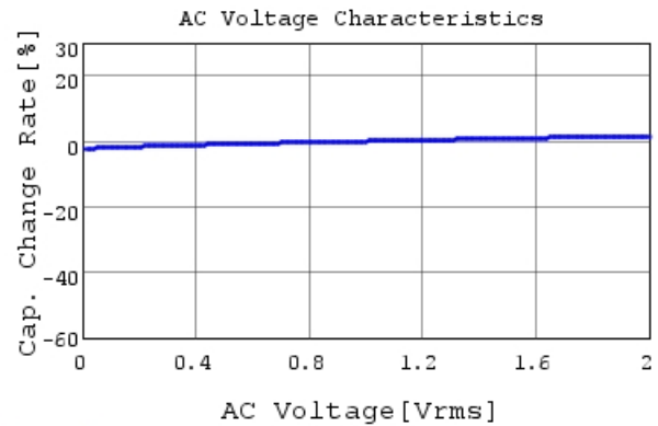
GRM55DR72A105KA01 C-AC Voltage capchange, Dc
