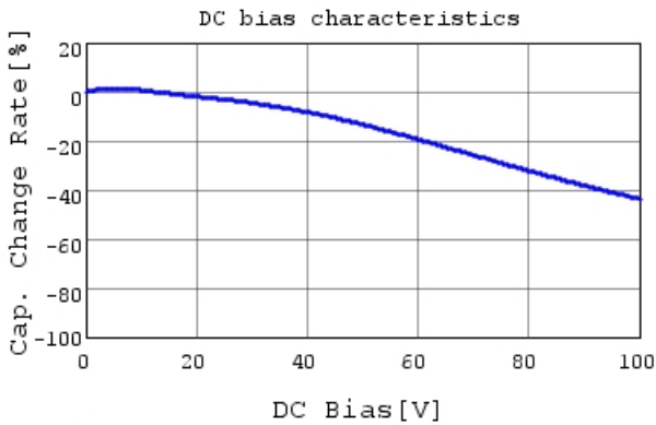
GRM55DR72A105KA01 C-DC bias capchange, 25.0c
