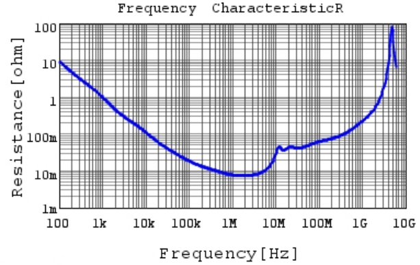
GRM55DR72A105KA01 R DCOV, 25degC
