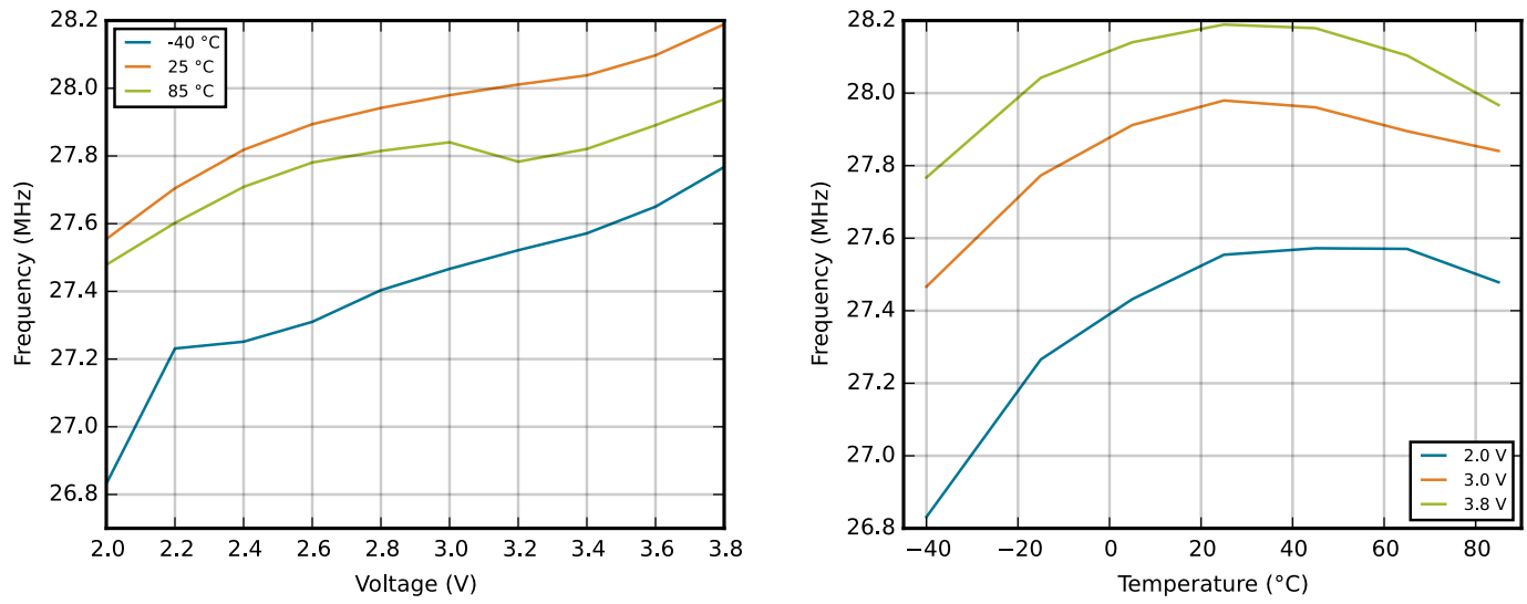
Figure 4.22. Calibrated HFRCO 28 MHz Band Frequency vs Supply Voltage and Temperature
