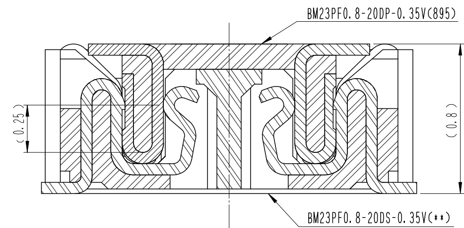
ENGAGEMENT FIGURE (50:1)
