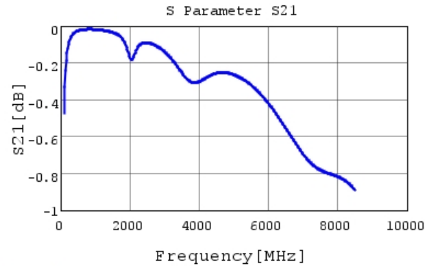
GRM1885C2A470JA01 S21 DCOV, 25degC
