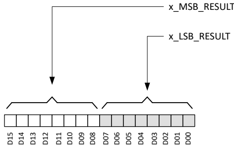
Figure 7-15. Magnetic Sensor Data Definition
