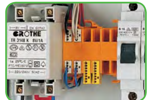
Example of doorbell application – mounted on DIN 35 rail
