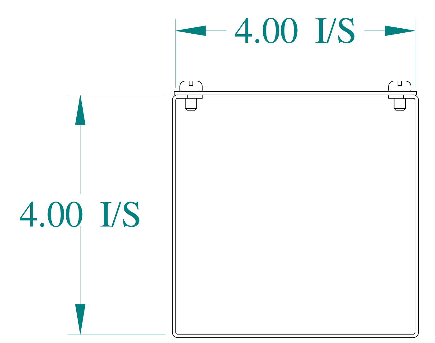
FRONT VIEW
