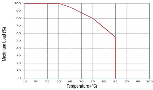
MTU2S0524MC
