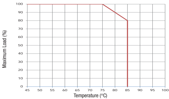
MTU2S2405MC
