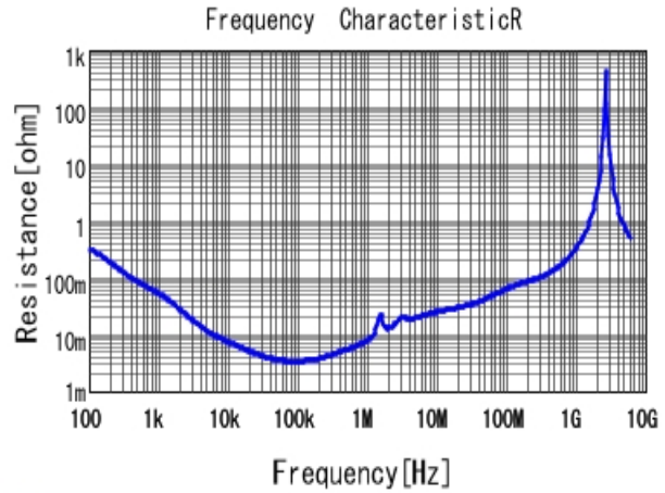
■ KCM55WR71J226MH01 R DCOV, 25degC
