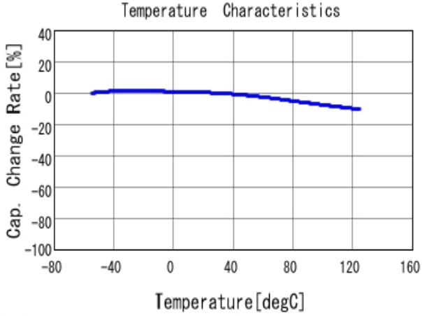
■ KCM55WR71J226MH01 C-Temp. capchange, DCOV, ACO, 5Vrms
