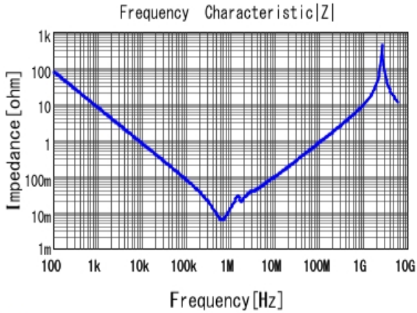
■ KCM55WR71J226MH01 |Z| DCOV, 25degC
