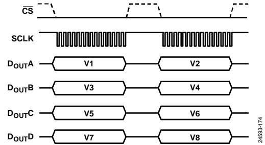
Figure 104. Serial Interface ADC Reading, Four D OUTX Lines
