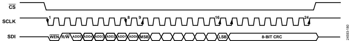
Figure 113. Writing Registers Through the SPI with CRC Enabled
