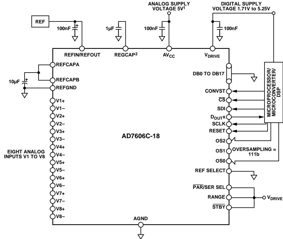
Figure 120. Typical Connection Diagram, Software Mode
