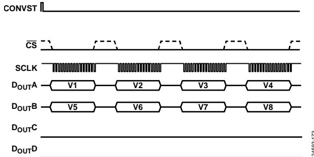
Figure 103. Serial Interface ADC Reading, Two D OUTX Lines
