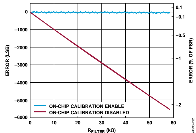
Figure 93. System Gain Calibration, with and Without Calibration, \pm 10 \text{ V} Single-Ended Range
