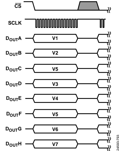
Figure 105. Serial Interface ADC Reading, Eight D OUTX Lines
