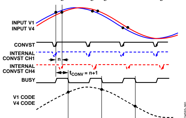
Figure 91. System Phase Calibration Functionality
