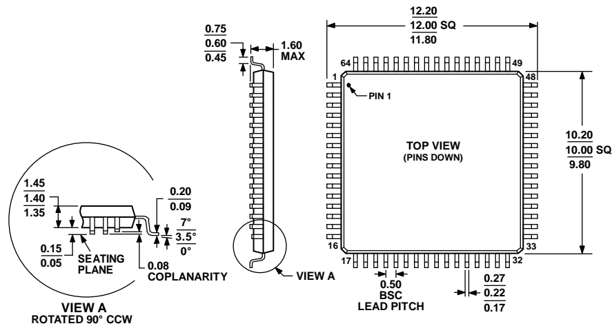
Figure 124. 64-Lead Low Profile Quad Flat Package [LQFP] (ST-64-2) Dimensions shown in millimeters
