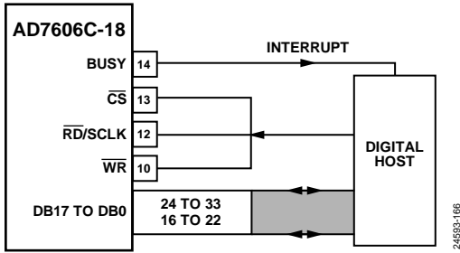
Figure 97. AD7606C-18 Interface Diagram—One AD7606C-18 Using the Parallel Bus with \overline{CS} and \overline{RD} Shorted Together
