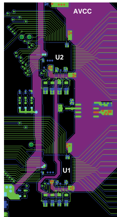
Figure 123. Layout for Multiple AD7606C-18 Devices—Top Layer and Supply Plane Layer
