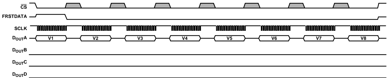
Figure 106. Serial Interface ADC Reading, One D OUTX Line
