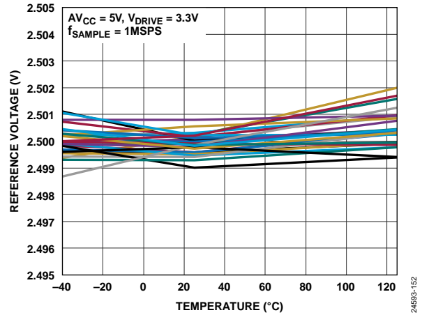
Figure 61. Reference Drift
