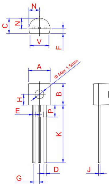
TO-92
