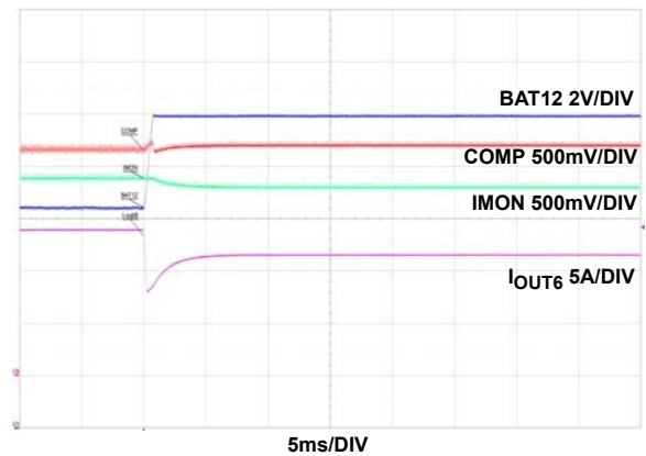
FIGURE 70B. RL = 0.10Ω → 0.15Ω
