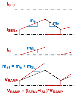
FIGURE 136. SLOPE COMPENSATION BLOCK DIAGRAM
