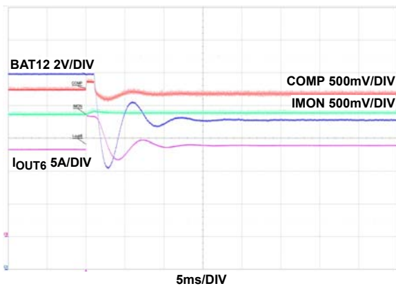
FIGURE 70A. RL1 = 0.15Ω → 0.1Ω
