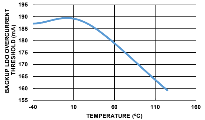
FIGURE 116. BACKUP LDO OVERCURRENT THRESHOLD vs TEMPERATURE, DEFAULT REGISTER SETTING
