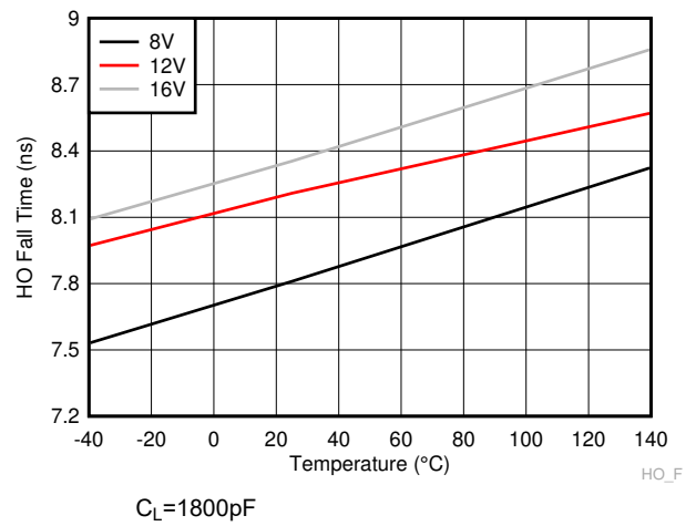
Figure 6-19. HO Fall Time
