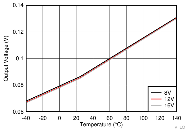
Figure 6-12. LO Low Output Voltage ( V_{LOL} ) I_O = 100\text{mA}
