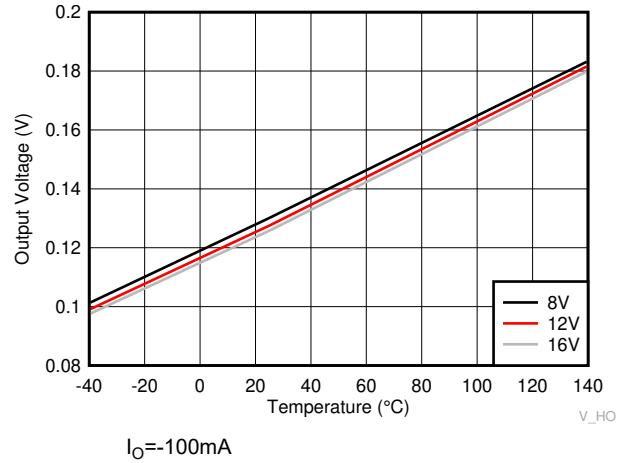
Figure 6-15. HO High Output Voltage ( V_{HOH} )
