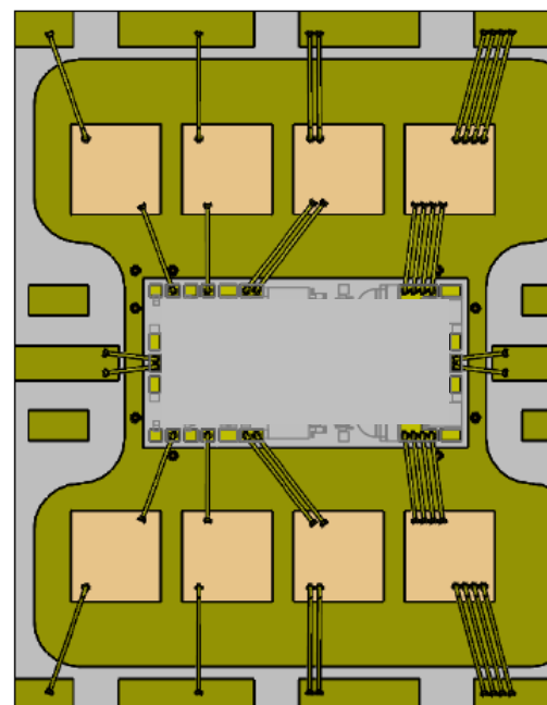
Die and capacitor placement and bonding detail
