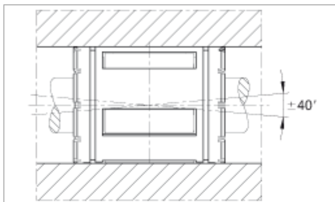
Self-aligning up to \pm 40'
