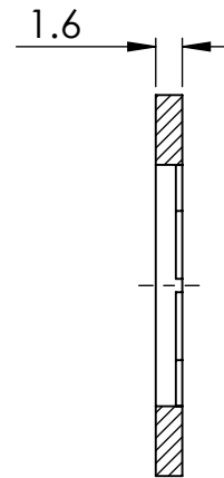
SECTION Y-Y
