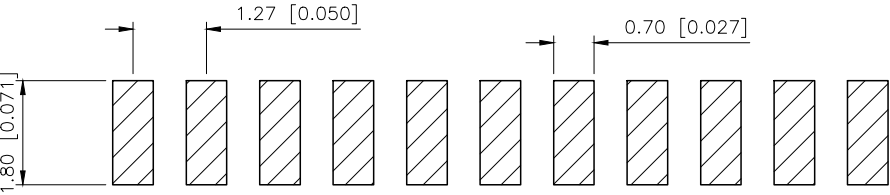
PCB LAYOUT
