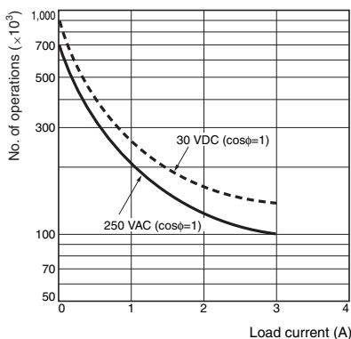
Resistive load
