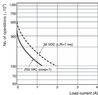
Inductive load
