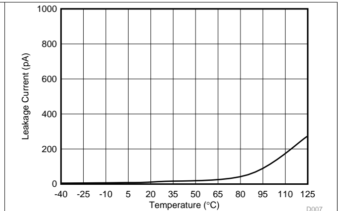
Figure 8. Leakage Current vs. Temperature
