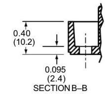
1, 3 & 5 Mount End
