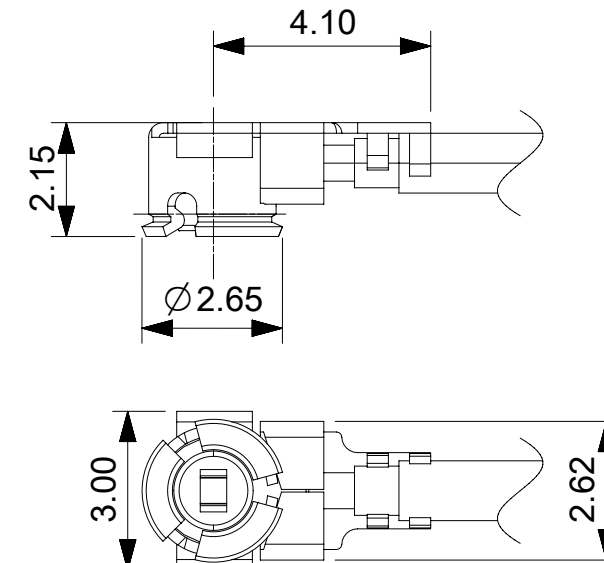
U.FL CONNECTOR
