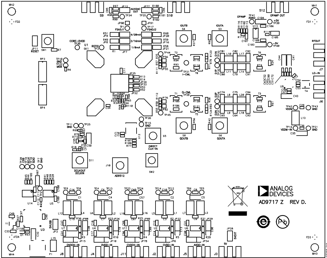
Figure 129. Silkscreen—Primary Side
