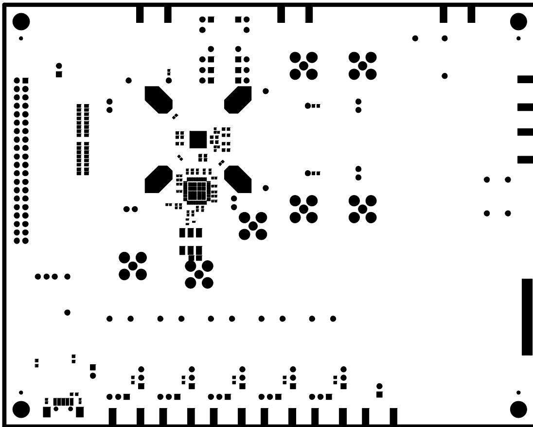
Figure 125. Solder Mask—Secondary Side
