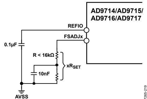
Figure 97. xR_{SET} Configuration for Values > 16 k \Omega
