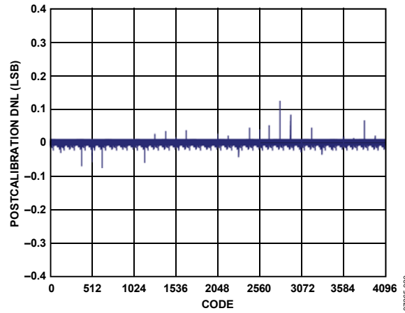
Figure 22. AD9716 Postcalibration DNL at 3.3 V
